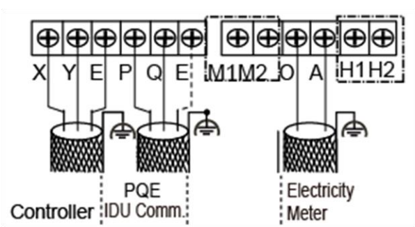
Figure 3-8.4: Outdoor unit communication terminals
