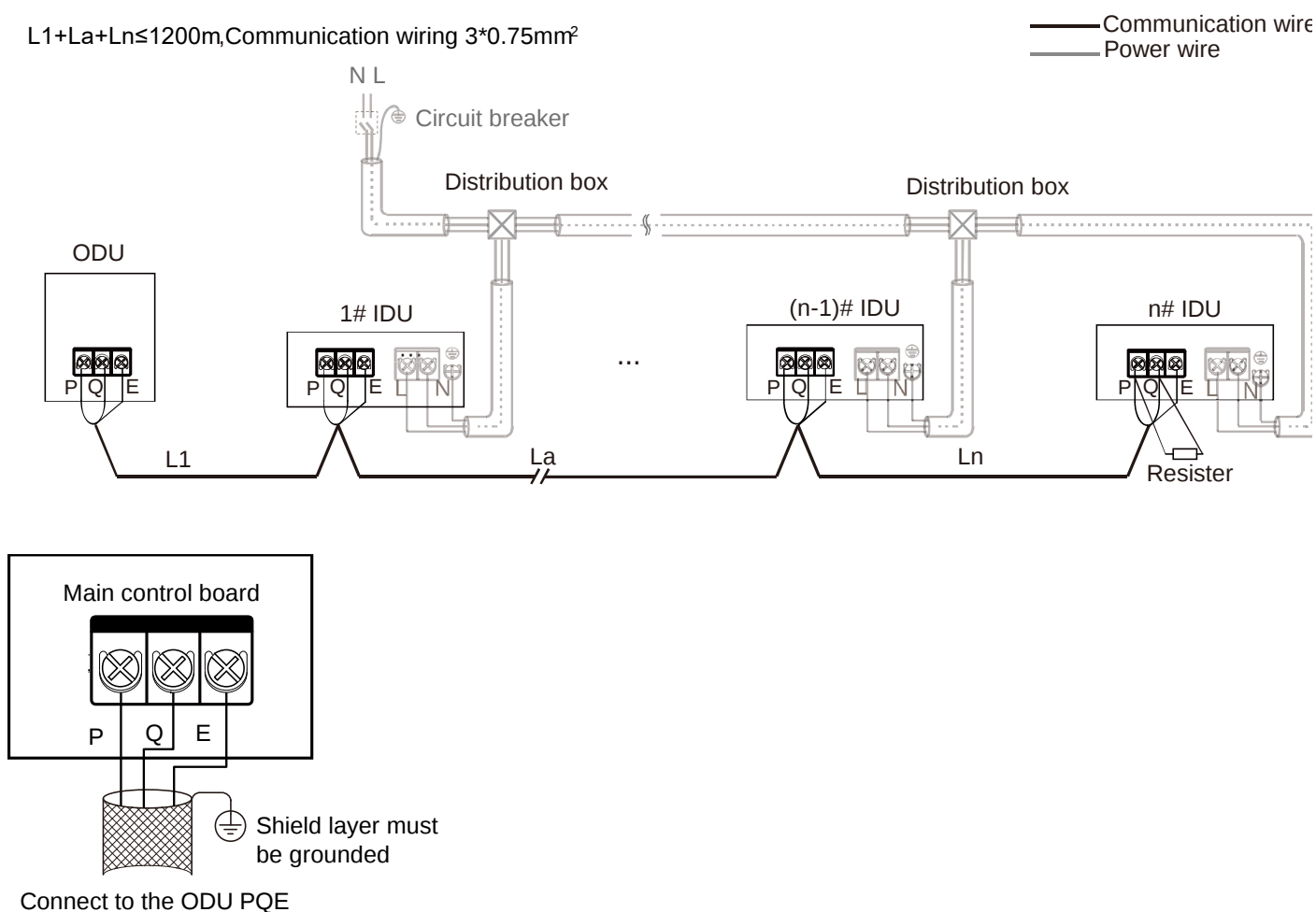
Figure 3-8.5: P Q E communication wiring configuration – IDUs unified power supplied
