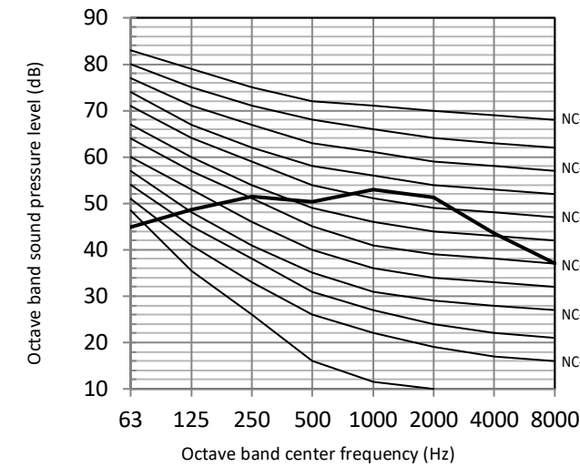
Figure 2-10.2: 120 model octave band level
