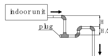
Figure 3-5.6: Drain piping water traps
