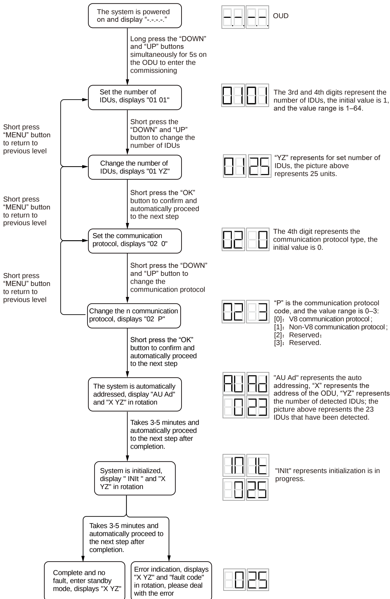
Figure 3-10.1: Test Run Procedure
